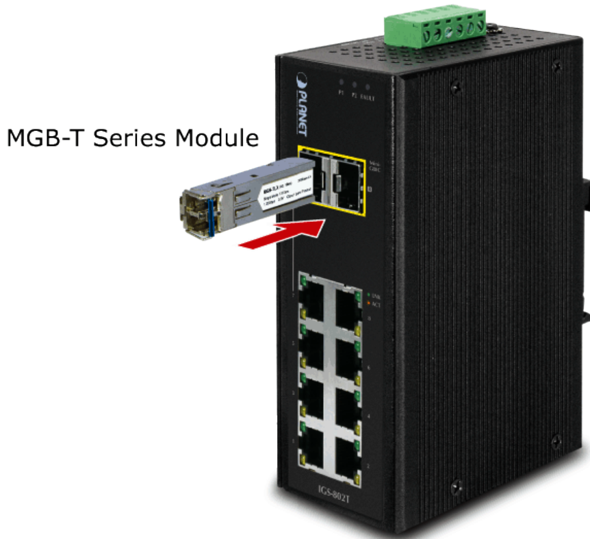
Figure 2-2-4a: Plug in the SFP Transceiver
