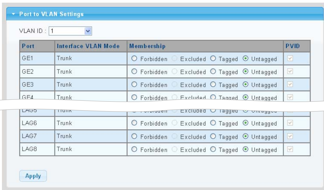
Figure 4-5-7 Port to VLAN Setting Page Screenshot
