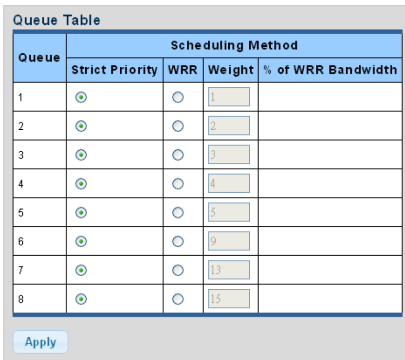
Figure 4-8-4 Queue Table Page Screenshot
