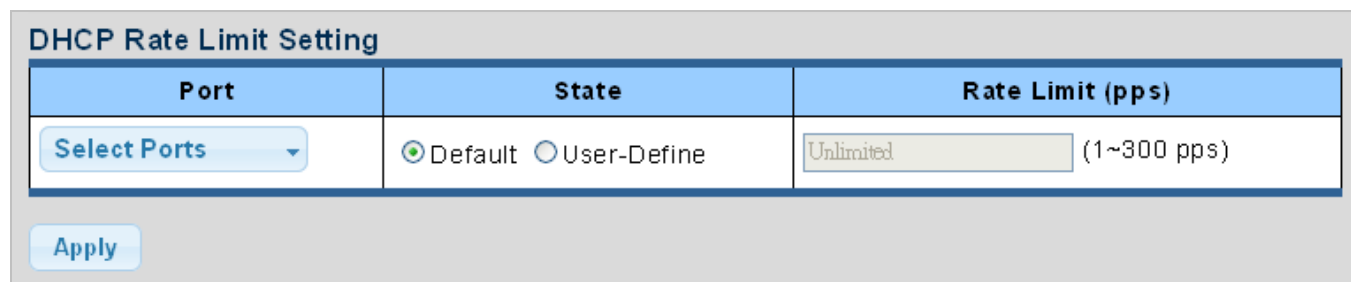
Figure 4-9-42 DHCP Rate Limit Setting Page Screenshot
