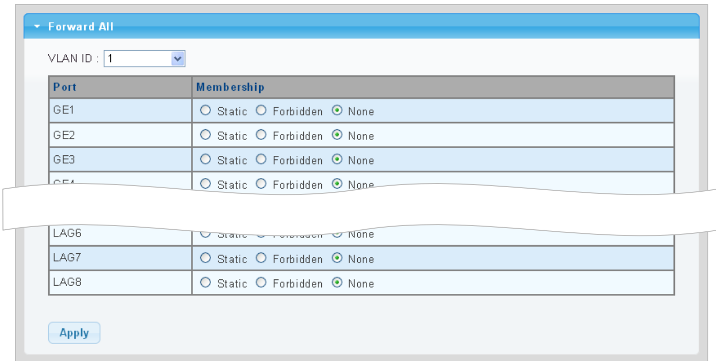
Figure 4-7-32 Forward All Setting Page Screenshot
