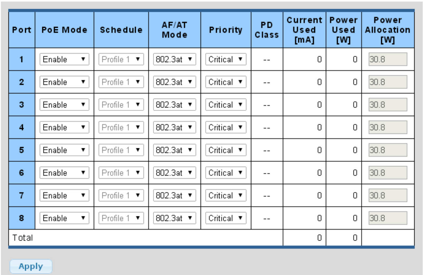
Figure 4-16-3: Power over Ethernet Configuration Screenshot
