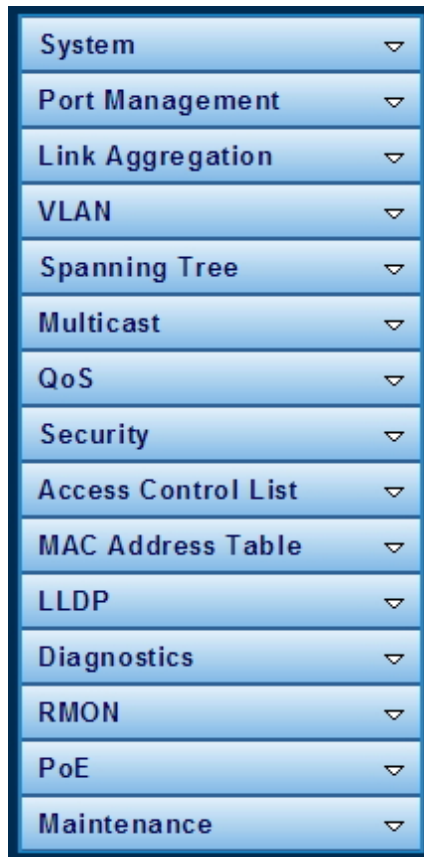
Figure 4-1-5 Industrial Managed Switch Main Functions Menu
