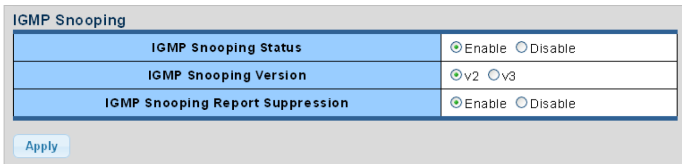
Figure 4-7-7 IGMP Snooping Page Screenshot
