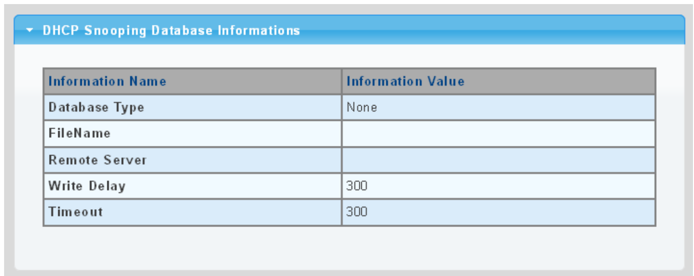
Figure 4-9-41 DHCP Snooping Database Information Page Screenshot
