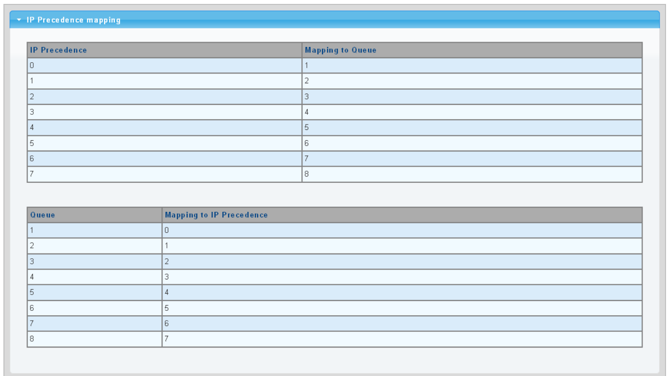
Figure 4-8-11 IP Precedence Mapping Page Screenshot
