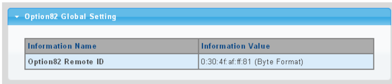
Figure 4-9-45 Option82 Global Setting Page Screenshot
