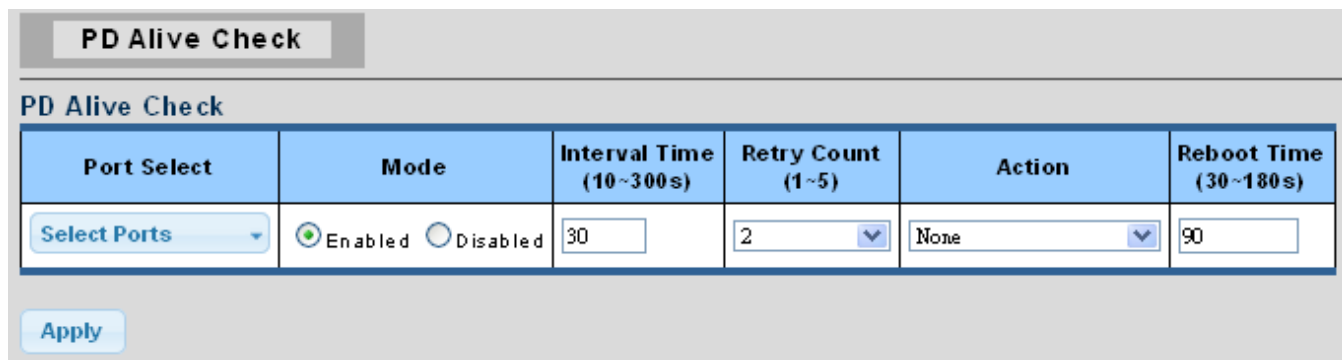
Figure 4-15-5: PD Alive Check Configuration Screenshot
