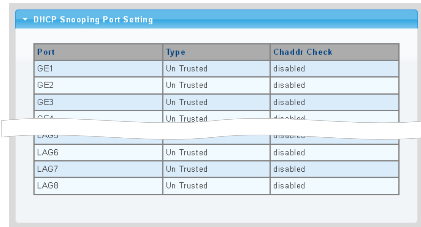
Figure 4-9-38 DHCP Snooping Port Setting Page Screenshot
